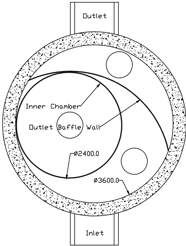
Plan
